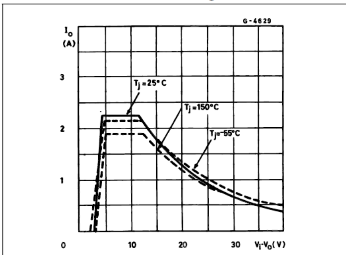
Figure 3. Output current vs input-output differential voltage
