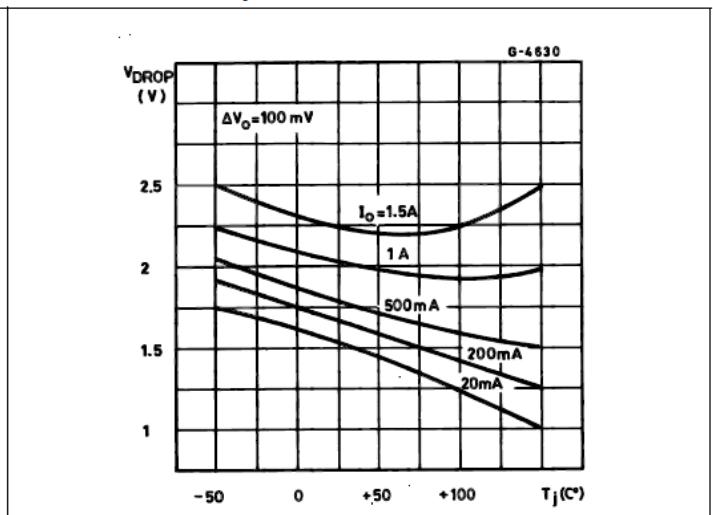
Figure 4. Dropout voltage vs junction temperature
